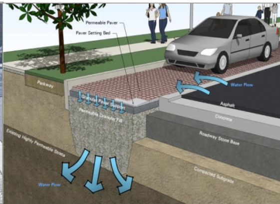
Permeable Pavement in Parking Lanes
