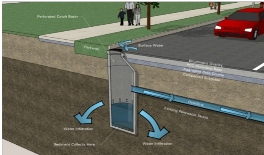
Perforated Catch Basins and Drywells
